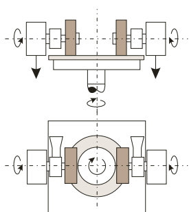
Tribometer-Test (view from the front side)
